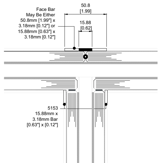
HORIZONTAL SECTION THROUGH 3-WAY DOUBLE/DOUBLE GLAZED JOINT
