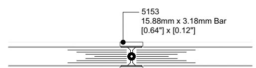
HORIZONTAL SECTION THROUGH SINGLE GLAZED BUTT JOINT
