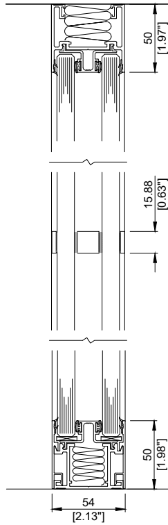
VERTICAL SECTION THROUGH DOUBLE GLAZED SHOREDITCH EDITION SCREEN
