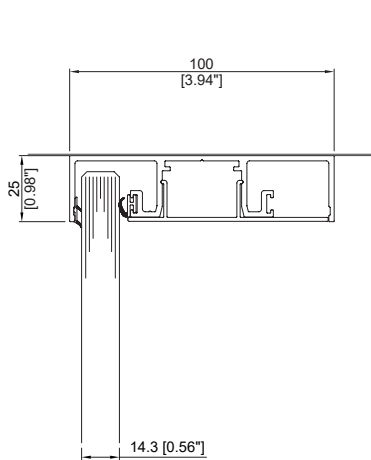
25mm [0.98"] HEAD TRACK OFFSET SINGLE GLAZED
