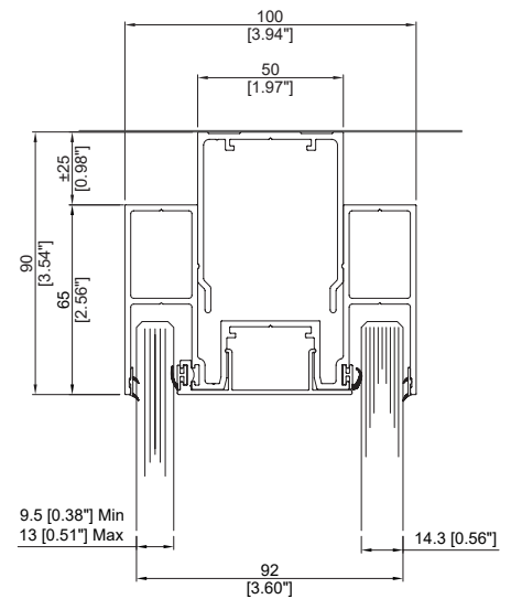
HEAD TRACK WITH INNER UPPER CHANNEL \pm 25 [0.98] DEFLECTION DOUBLE GLAZED
