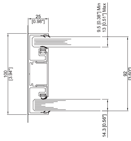
25mm [0.98"] ABUTMENT FIXED GLAZING BEAD DOUBLE GLAZED
